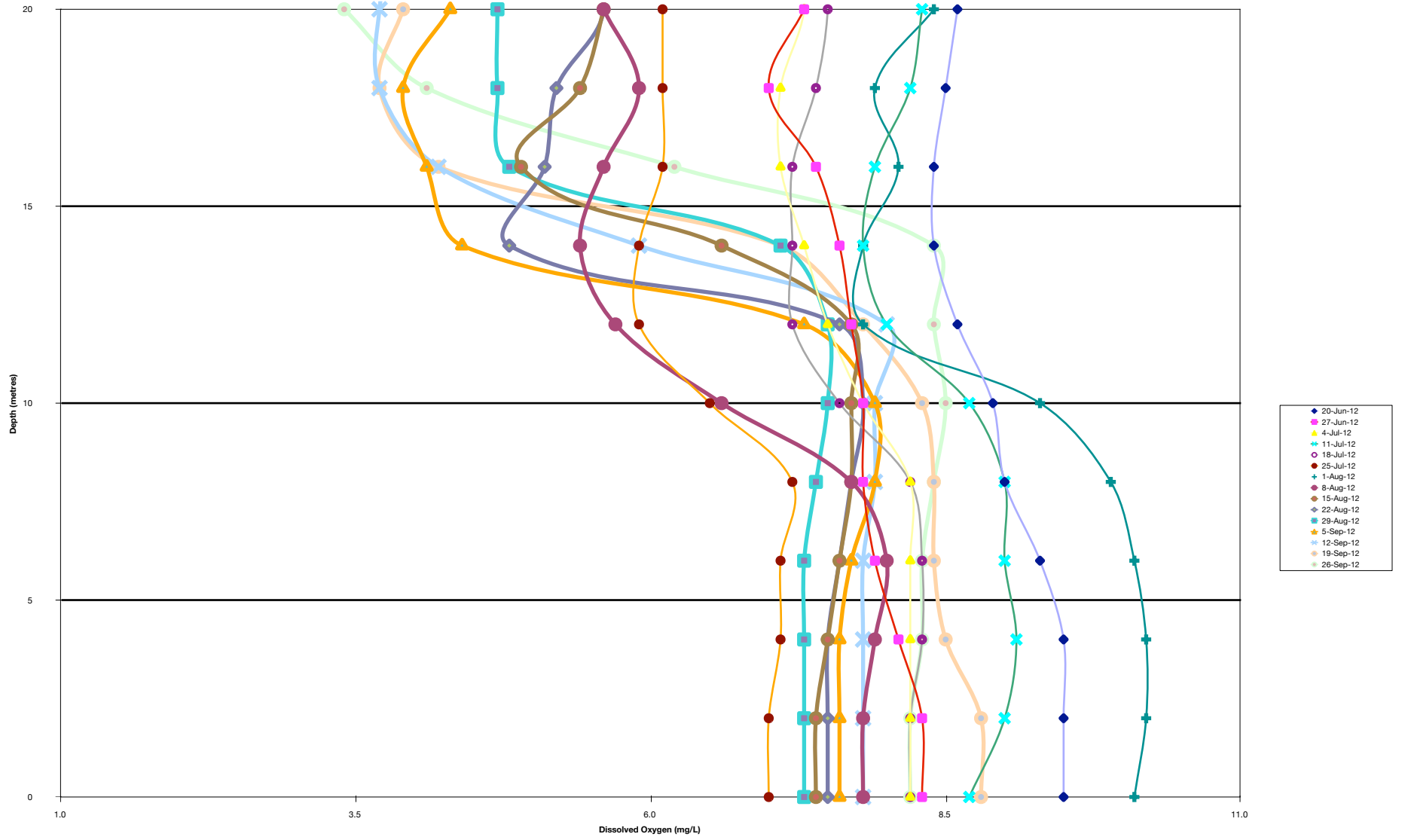
Osoyoos Lake (at White Sands) - Oxygen Profiles 2012
