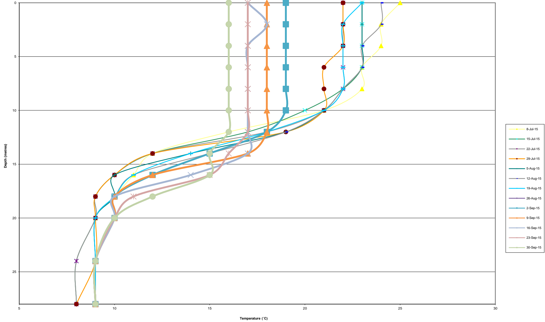
Osoyoos Lake (at Packinghouse) - Temperature Profiles 2015
