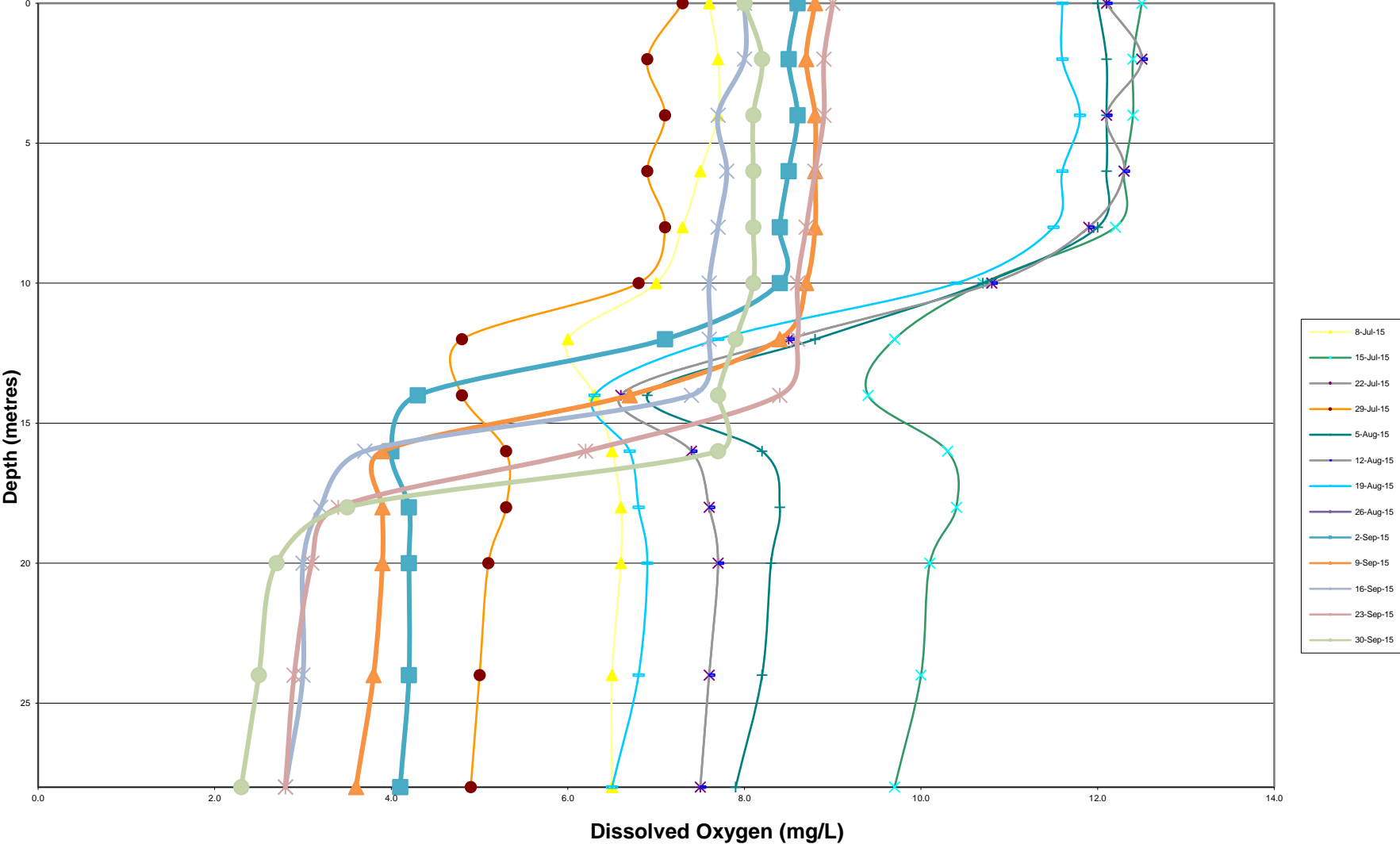
Osoyoos Lake (at Packinghouse) - Oxygen Profiles 2015
