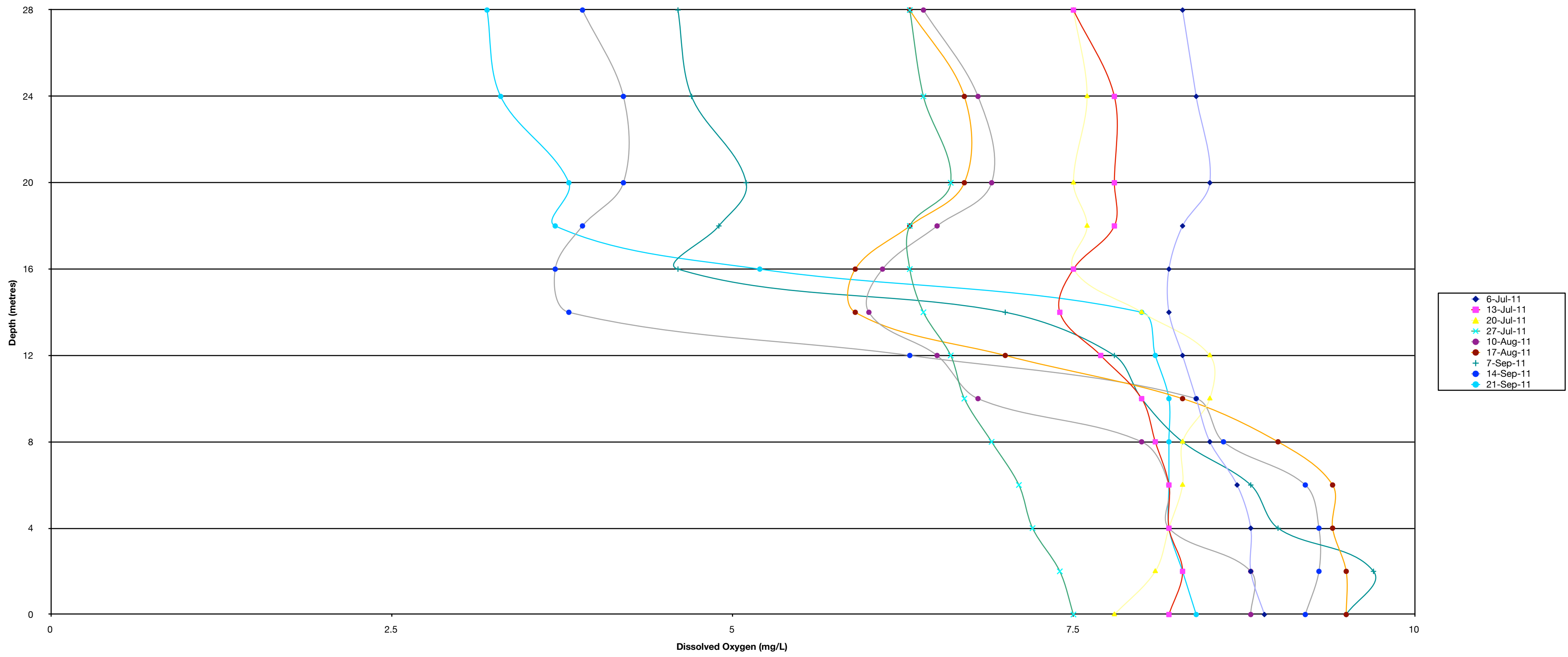
Osoyoos Lake (at North End) - Oxygen Profiles 2011
