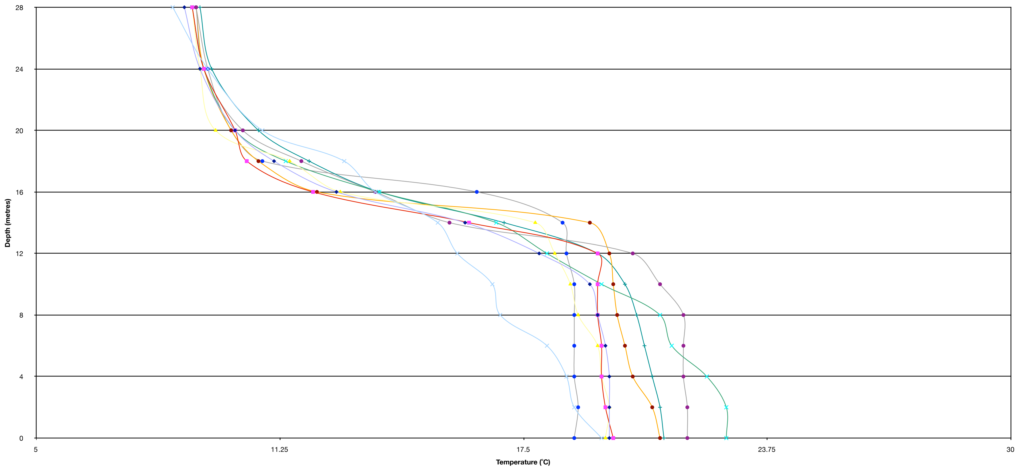
Osoyoos Lake (at North End) - Temperature Depth Profiles 2011
